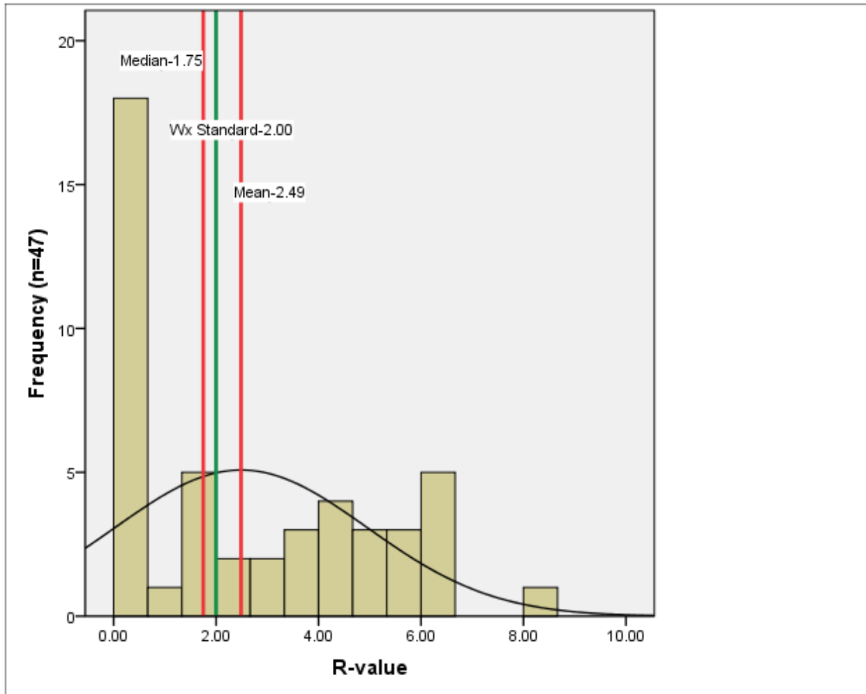
Figure A-8: Distribution of Duct Insulation R-Values in Unconditioned Basements (Base: All homes with ducts in unconditioned basements)
