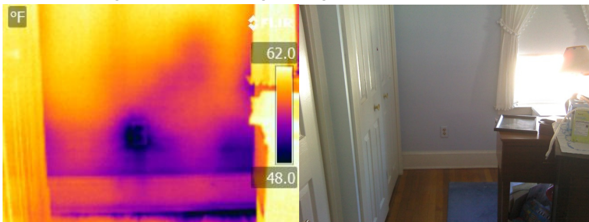
Figure D-21: Air Leakage through Baseboard and Outlet
