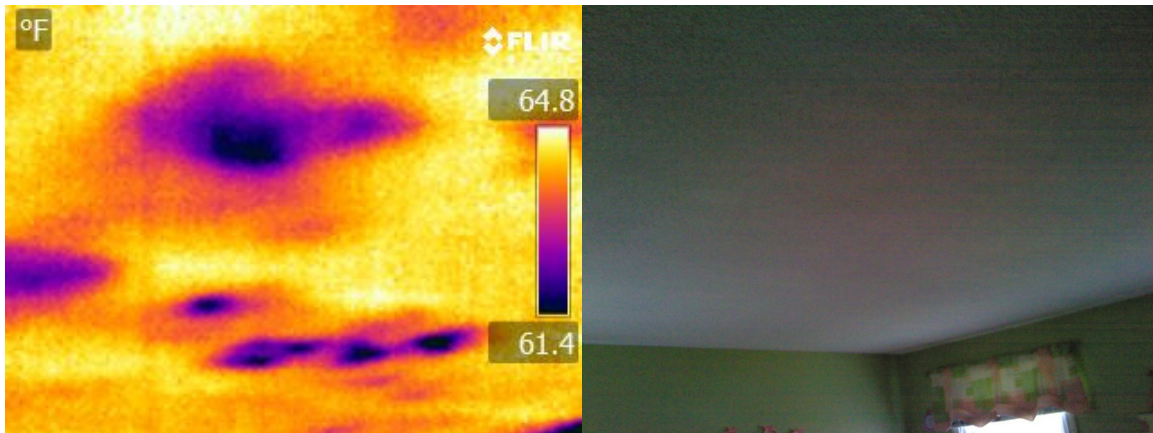
Figure D-30: Missing Attic Insulation
