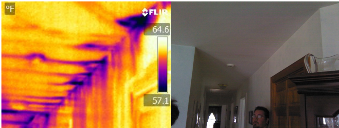
Figure D-16: Air Leakage at Attic Top Plate
