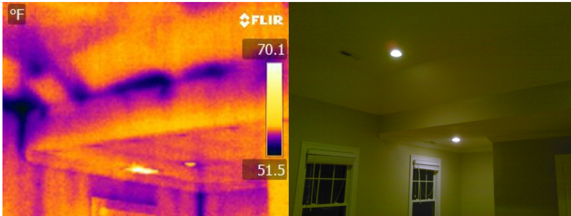
Figure D-34: Poor Insulation Installation in Tray Ceiling
