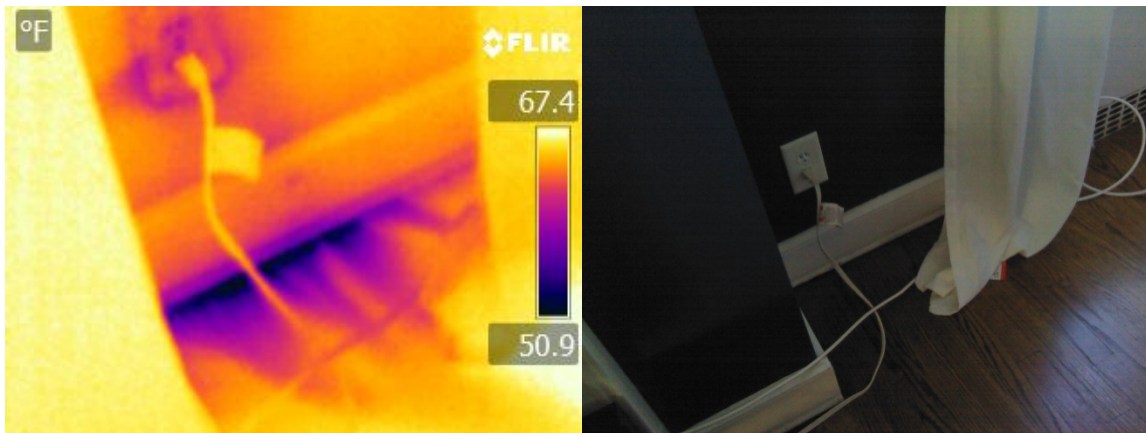
Figure D-20: Air Leakage at Baseboard Trim
