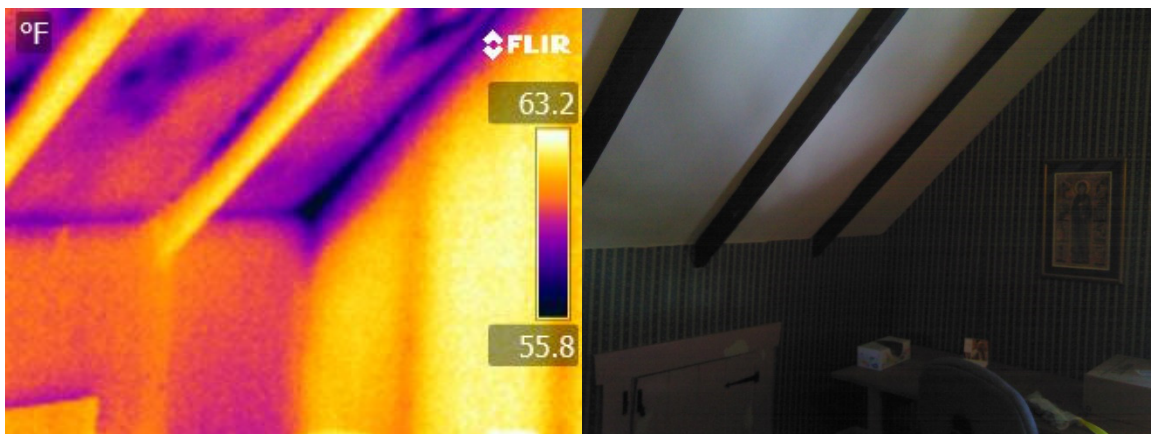
Figure D-33: Old, Inconsistent Vaulted Ceiling Insulation
