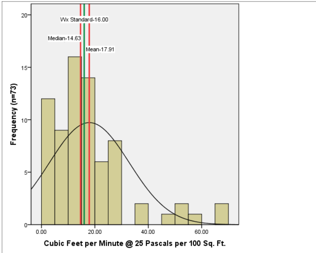
Figure A-7: Distribution of Duct Leakage to the Outside Results (CFM25/100 sq. ft.) (Base: All homes where duct leakage to the outside was tested)
