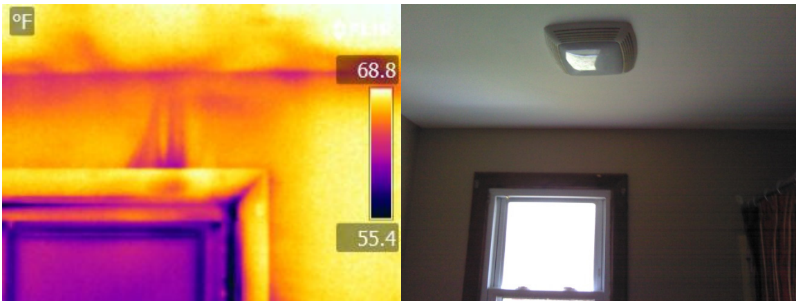
Figure D-23: Air Leakage at Framing around Window
