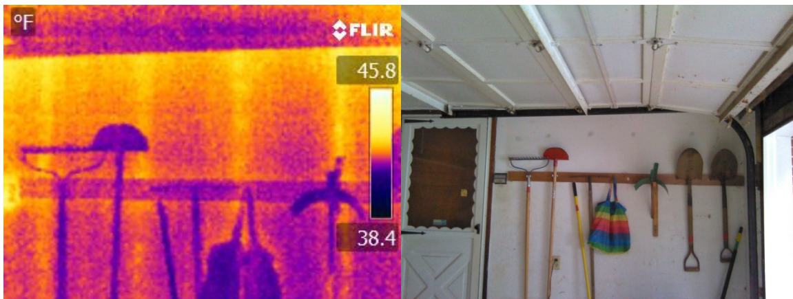
Figure D-29: Settling of Blown-In Cellulose Insulation
