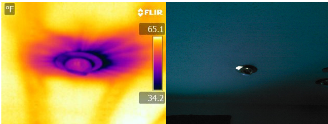
Figure D-25: Air Leakage at a Recessed Light Fixture
