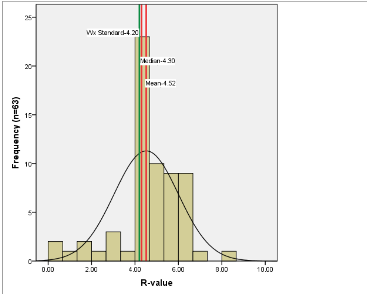
Figure A-9: Distribution of Duct Insulation R-Values in Attics and Crawlspaces (Base: All homes with ducts in attics or crawlspaces)
