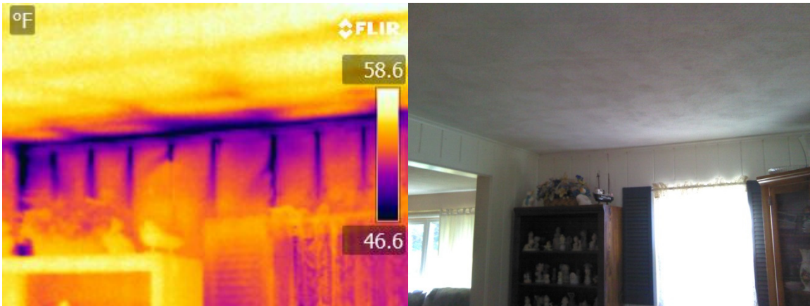
Figure D-3: Air Leakage at Top Plate of Exterior Wall
