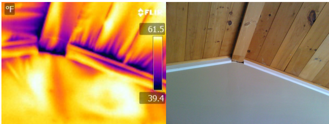
Figure D-17: Air Leakage through Ceiling Framing
