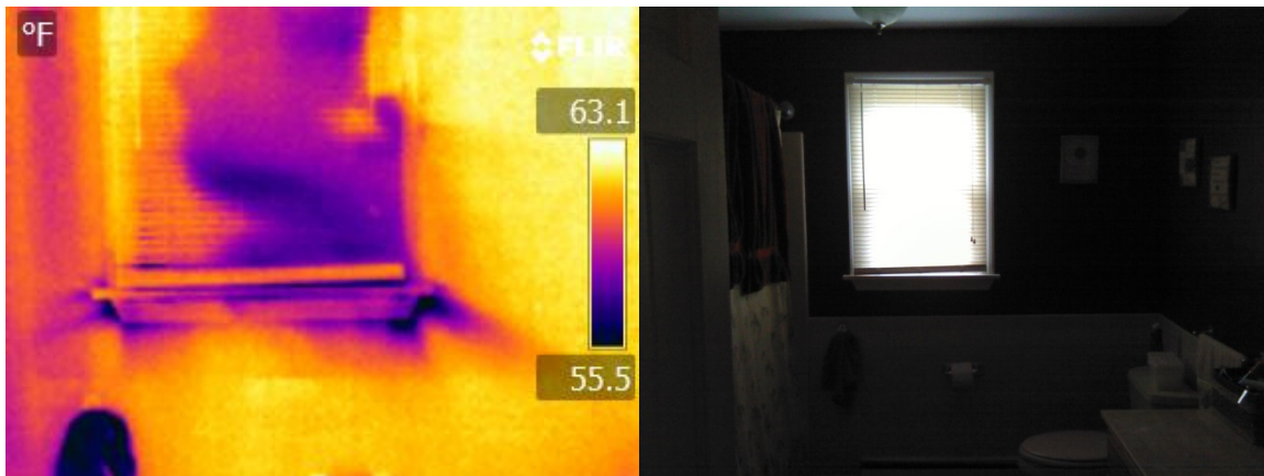
Figure D-24: Air Leakage at Framing around Bathroom Window
