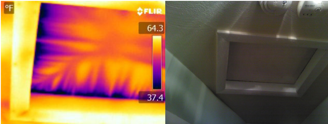
Figure D-22: Air Leakage through an Attic Hatch
