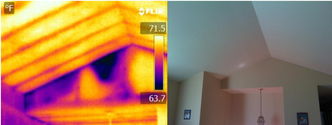
Figure D-26: Missing Knee Wall Insulation
