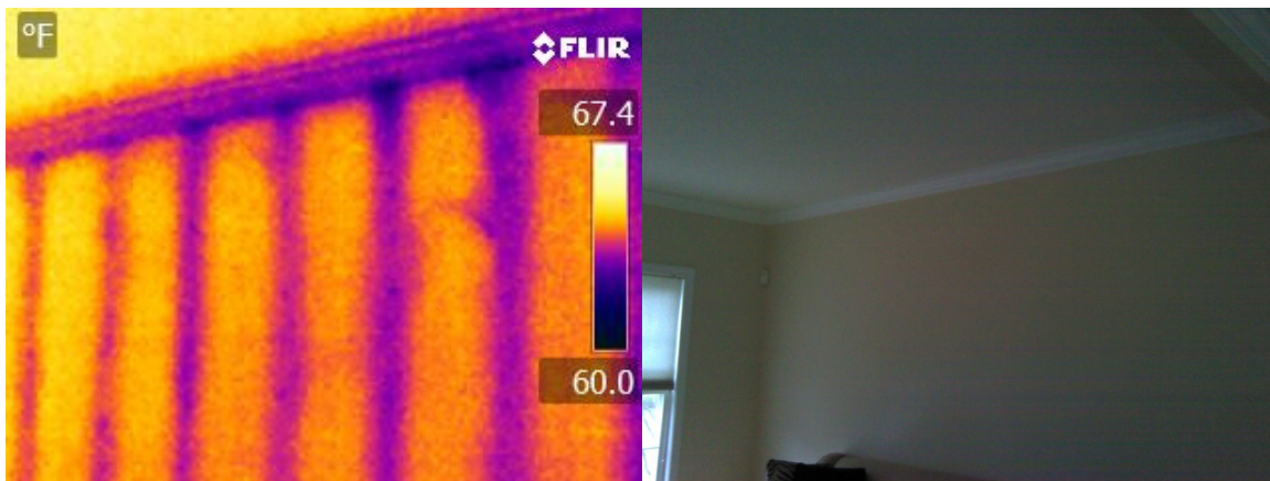
Figure D-36: Well Installed Wall Insulation
