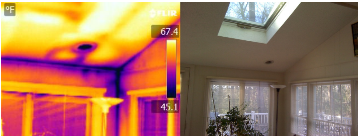
Figure D-18: Air Leakage at Top Plate and Vaulted Ceiling
