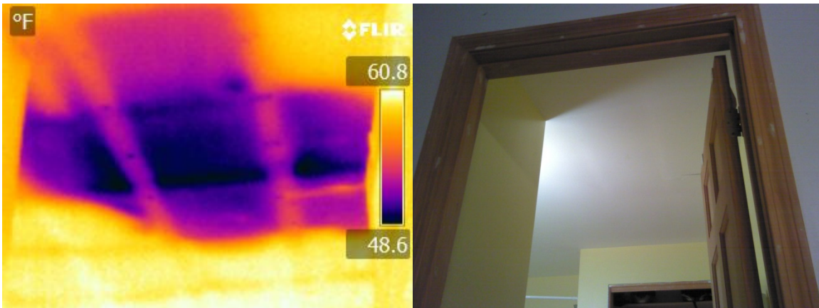
Figure D-27: Missing Attic Insulation
