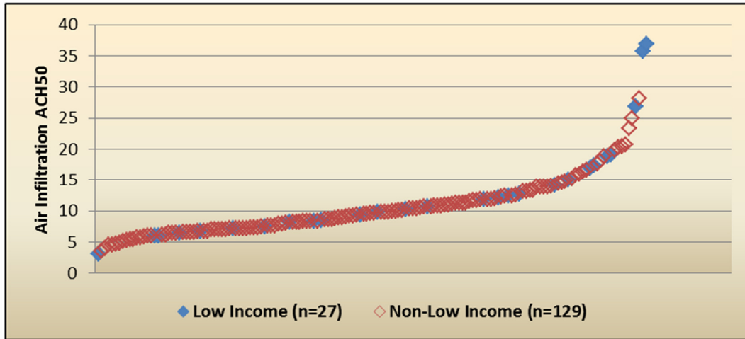
Figure 7-1: Air Changes per Hour at 50 Pascals—Low-Income vs. Non-Low-Income Homes
