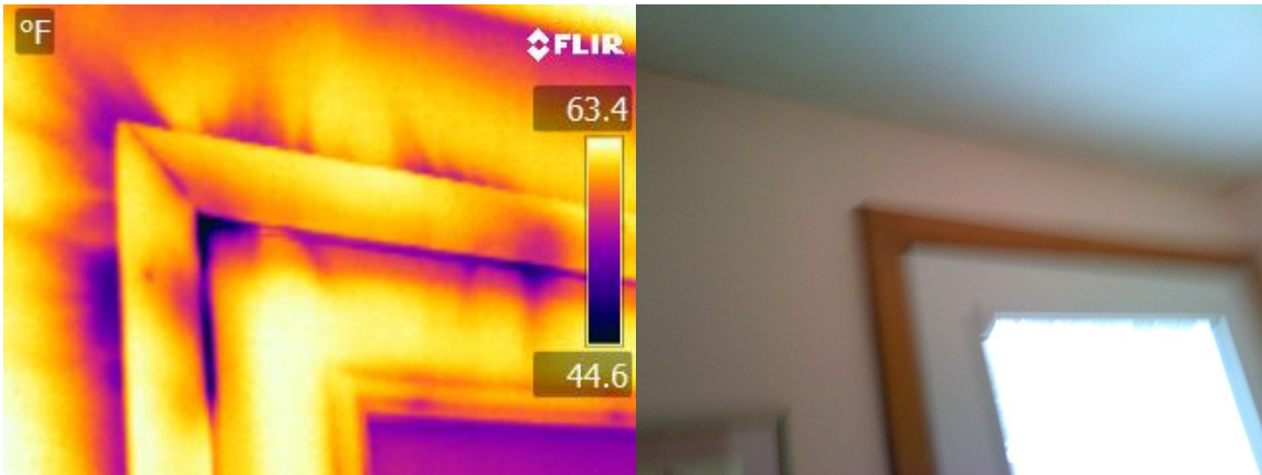
Figure D-19: Air Leakage at an Exterior Door
