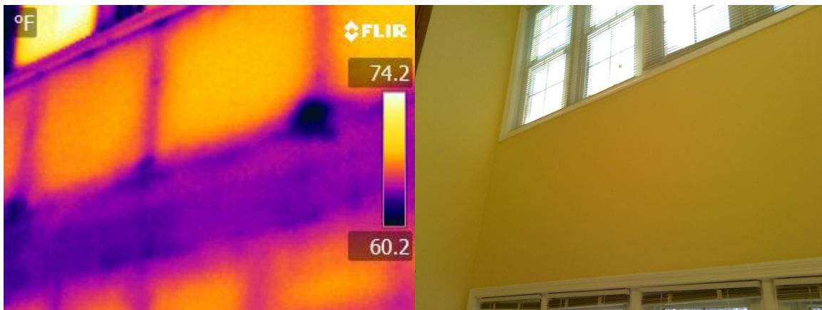
Figure D-31: Uninsulated Band Joist
